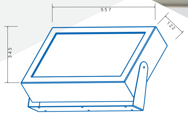
ML 505/22" dimensions
