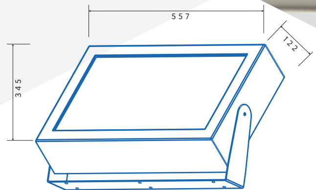
ML 505/22" dimensions
